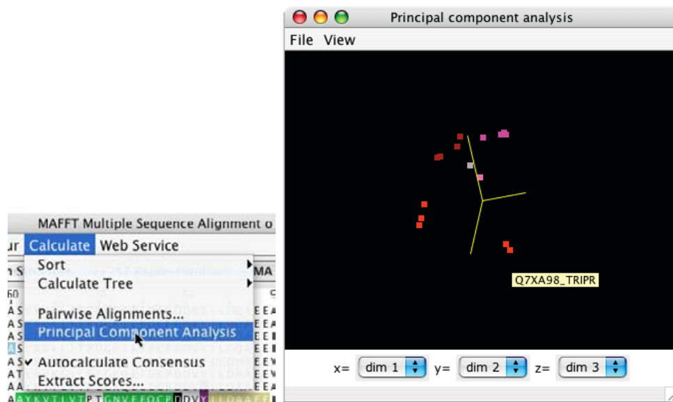
Figure 2.7: PCA Analysis
