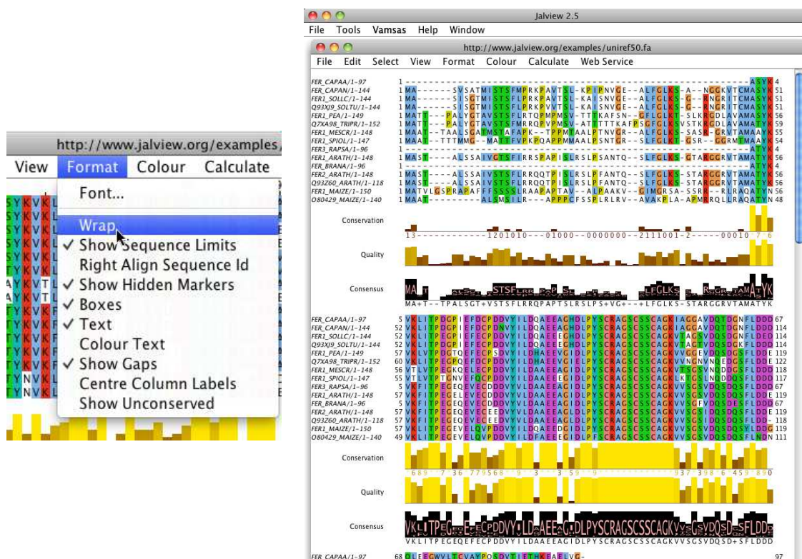
Figure 3.4: Wrapping the alignment.
