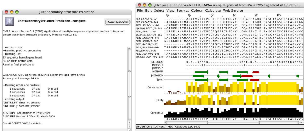
Figure 8.1: Secondary Structure Prediction Status (left) and results (right) windows for JPred predictions.
