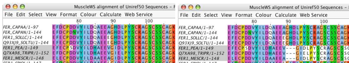
Figure 2.10: Introducing gaps in a group. Gaps are introduced as the selected group is dragged to the right with [CTRL] pressed.
