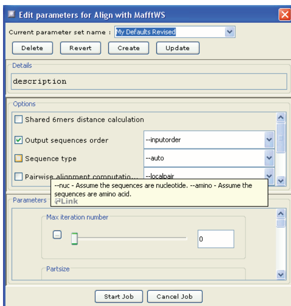
Figure 5.2: Jalview's JABA alignment service parameter editing dialog box.
