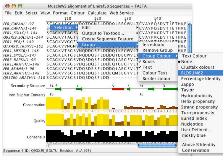
Figure 3.1: Colouring a group via the context menu.
