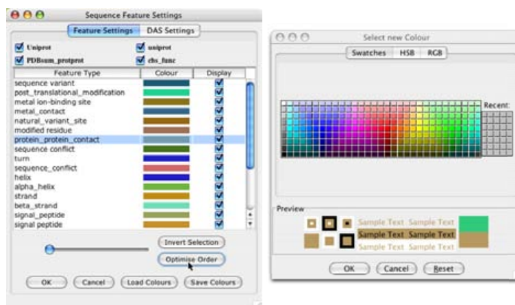
Figure 2.12: Customising sequence features. Features can be recoloured, switched on or off and have the rendering order changed.
