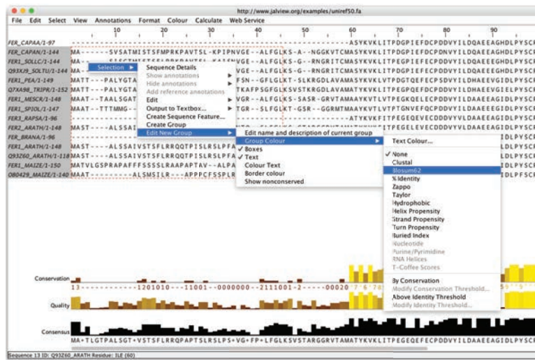
Figure 3.1: Colouring a group via the context menu.
