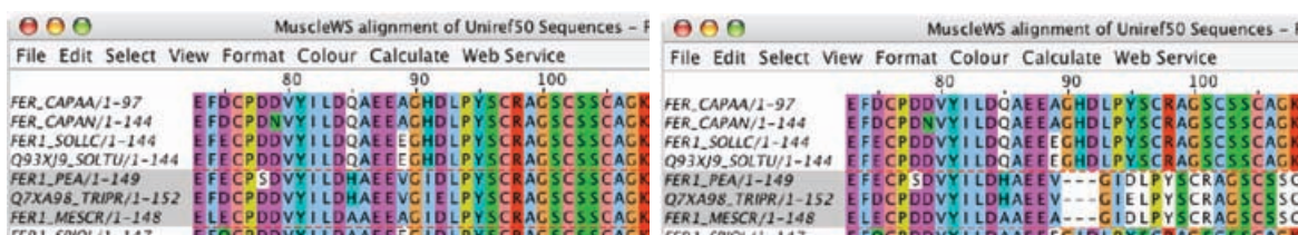
Figure 1.22: Introducing gaps in a group. Gaps are introduced as the selected group is dragged to the right with [CTRL] pressed.
