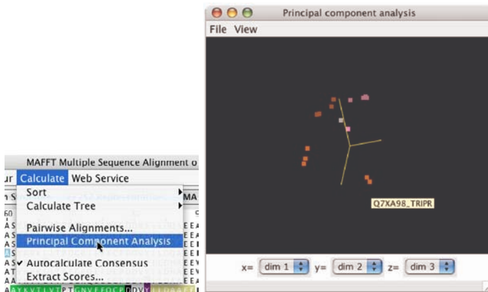
Figure 2.3: PCA Analysis
